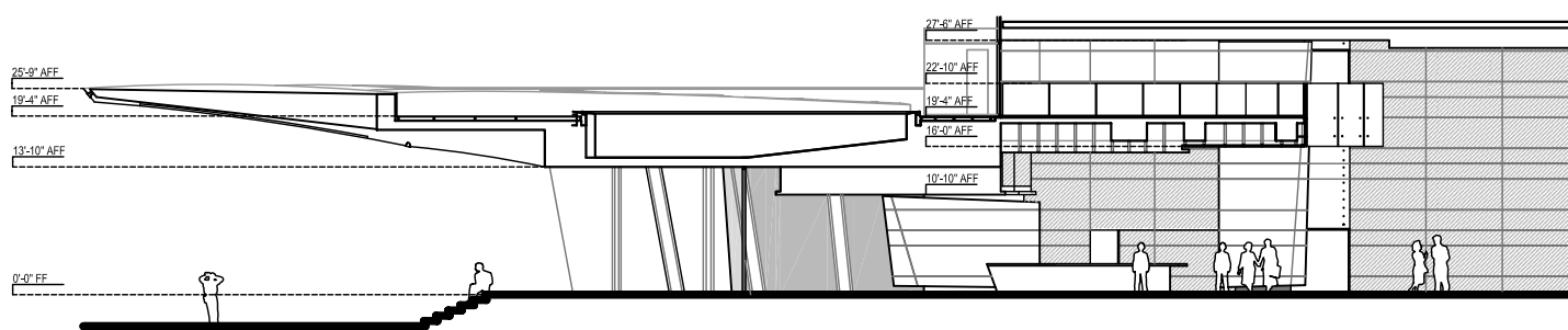
NORTH ACCESS LOBBY INTERIOR ELEVATION B
